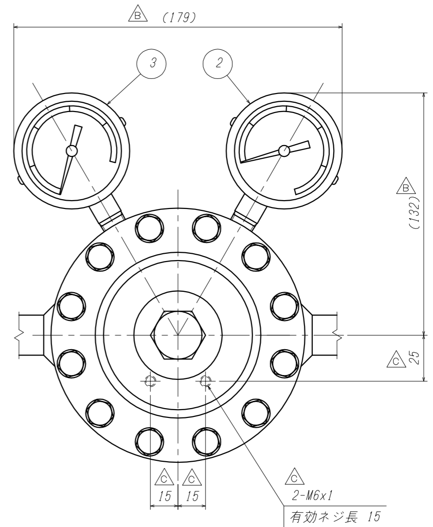
View A
